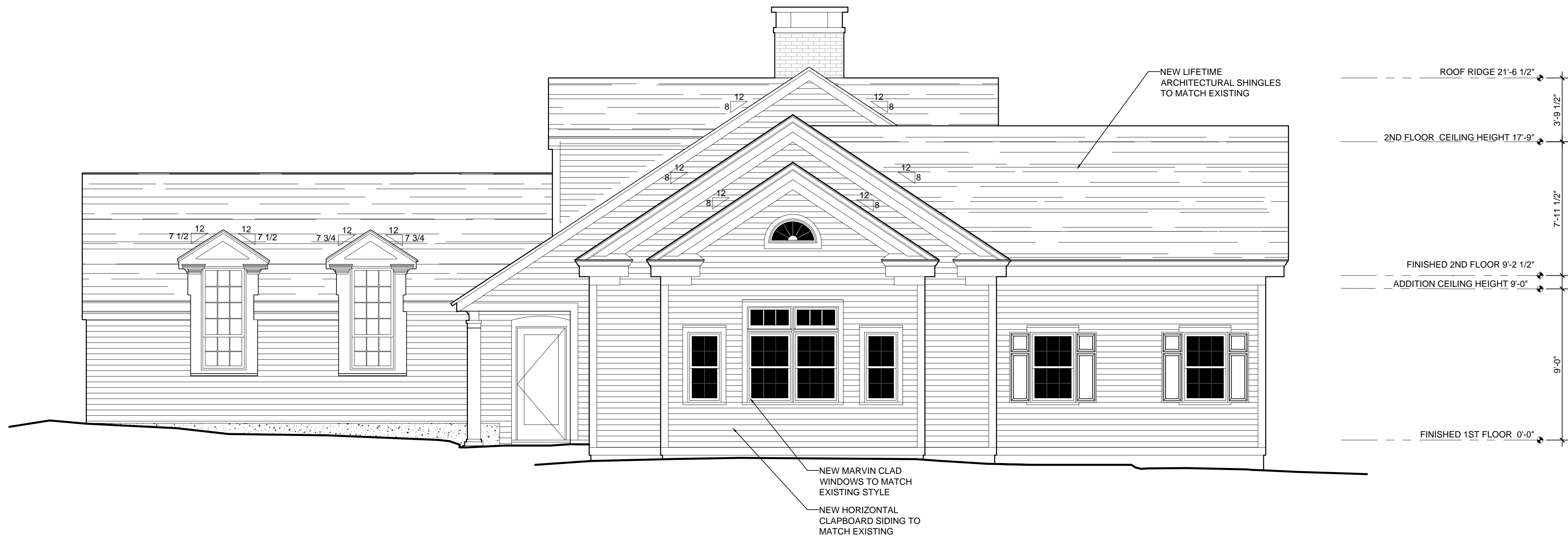
1 WEST ELEVATION SCALE: 1/4"=1'
